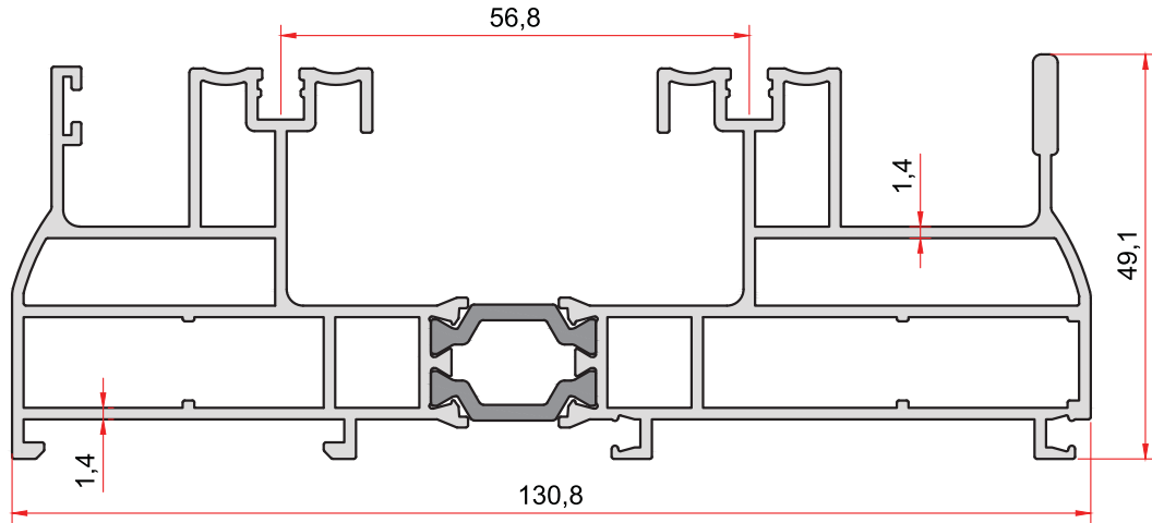
KOD-CODE TEORİK AĞIRLIK THEORETICAL WEIGHT SS-102-14 2,678 Kg/m
