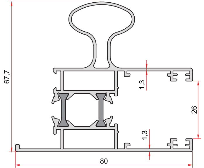
KOD-CODE TEORİK AĞIRLIK THEORETICAL WEIGHT SS-204-13 1,556 Kg/m
