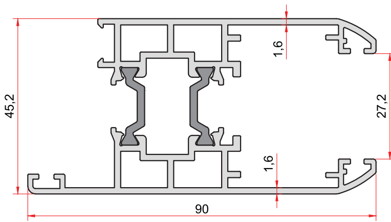
KOD-CODE TEORİK AĞIRLIK THEORETICAL WEIGHT SS-202-16 1,786 Kg/m
