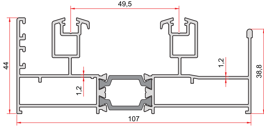
KOD-CODE TEORİK AĞIRLIK MD-103-12 THEORETICAL WEIGHT 1,825 Kg/m
