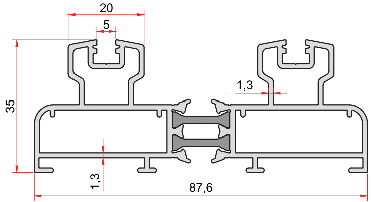
KOD-CODE TEORİK AĞIRLIK THEORETICAL WEIGHT SS-103-13 1,529 Kg/m
