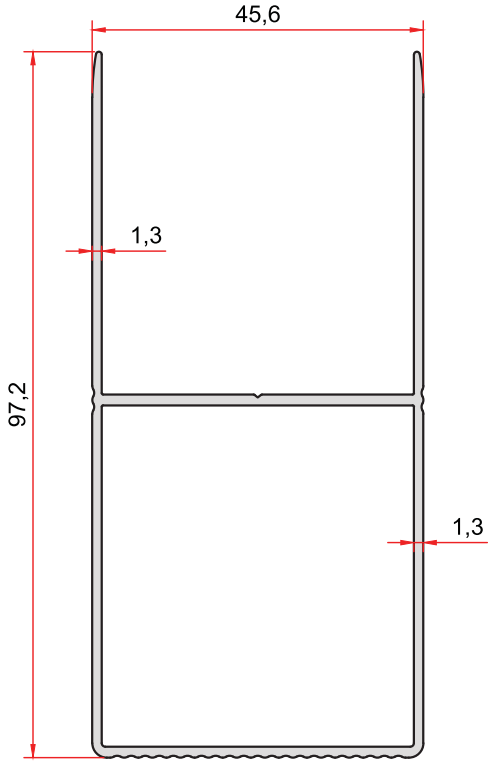
KOD-CODE TEORİK AĞIRLIK THEORETICAL WEIGHT 2666 1,002 Kg/m
